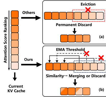
Figure 2: Existing methods (a) vs. D 2 O (b) at token level.
