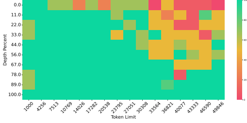
(c) 50k long-context fact retrieval of H 2 O method.
