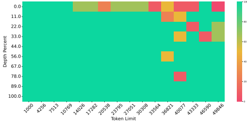
(e) 50k long-context fact retrieval of our D 2 O.
