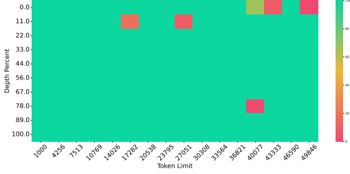
(a) 50k long-context fact retrieval of Full model.
