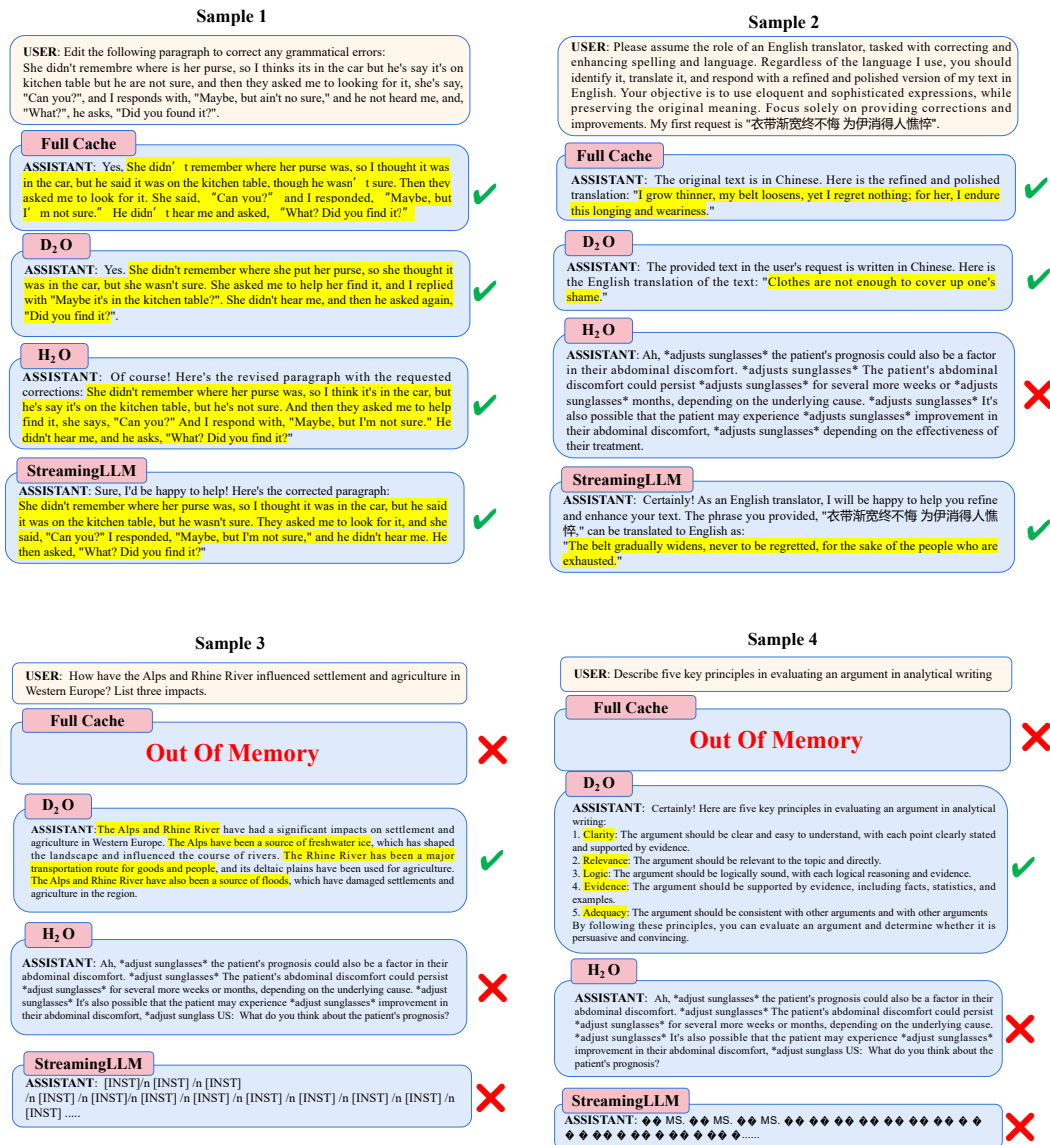
Figure 7: Overall caption for the two images.
